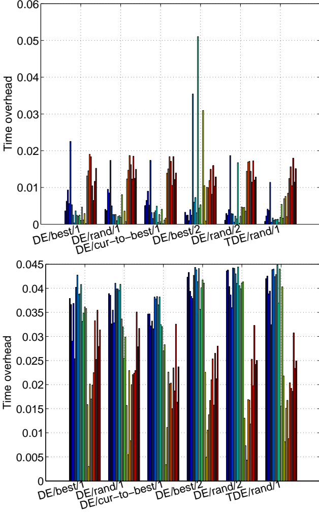
Figure 5: Computational time overhead of the proposed hybrid DE strategies against the \chi PSO algorithm on the 30-dimensional versions (top) and the 50-dimensional versions (bottom) of the CEC 2005 suite.
