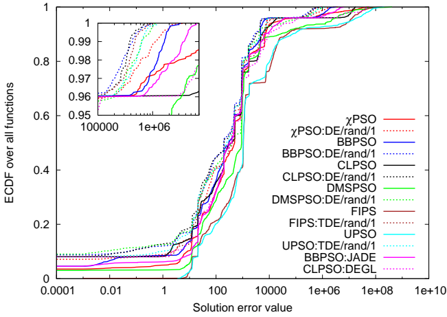
Figure 7: Empirical cumulative probability distribution of the solution error for the state of the art PSO variants against the corresponding hybrid frameworks on the CEC 2005 benchmark functions.
