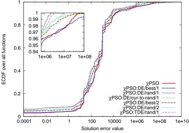
Figure 6: Empirical cumulative probability distribution of the solution error values for the local version of the \chi PSO algorithm against the corresponding hybrid DE variants on the 30 and 50-dimensional versions of the CEC 2005 benchmark functions.
