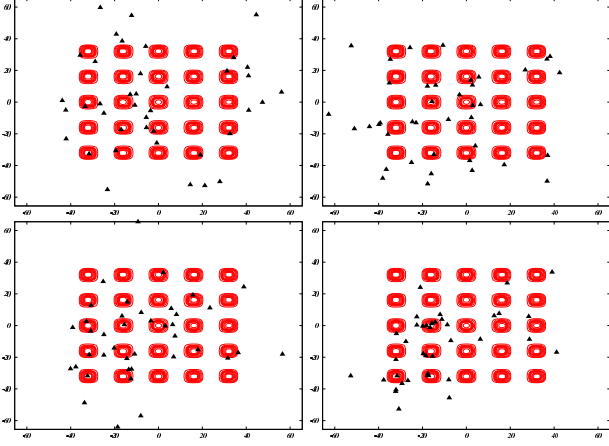
Figure 2: Local PSO population's positions after 1, 5, 10, and 20 generations
