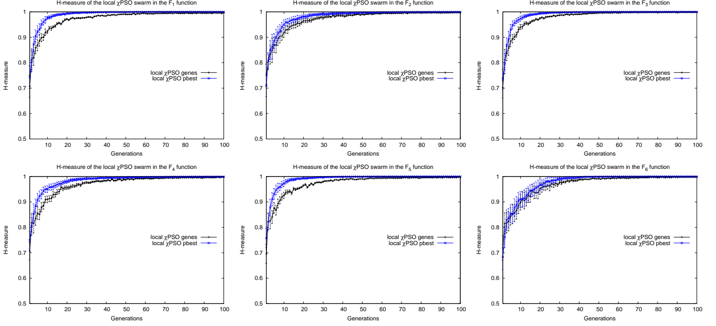
Figure 4: H-measure of the local \chi PSO for the six shifted benchmark functions
