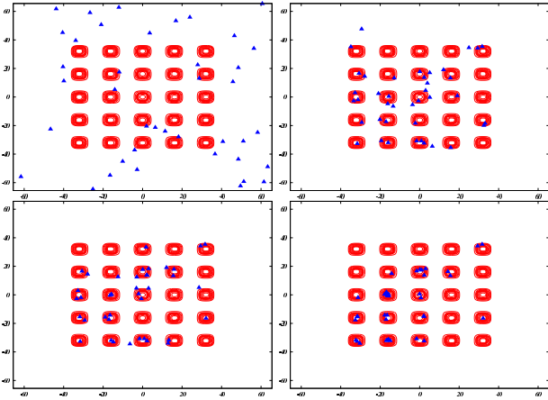
Figure 3: local PSO population's best personal positions after 1, 5, 10, and 20 generations
