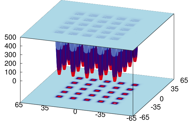
Figure 1: 3-D Plot of the Shekel's Foxholes function
