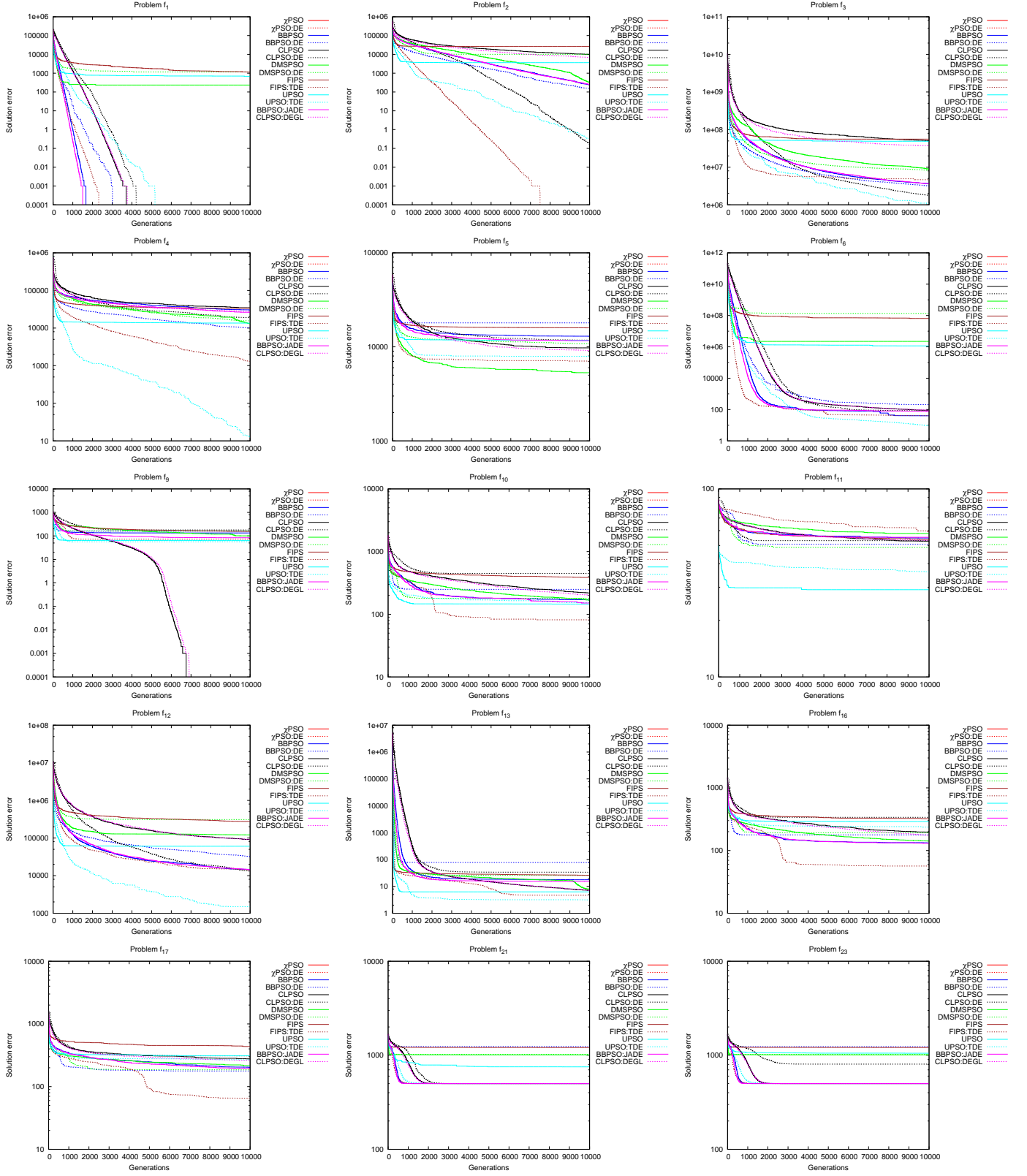
Figure 8: Convergence graph (median curves) for all PSO variants and their corresponding best performing hybrids on the 50-dimensional f_1 - f_6, f_9 - f_{13}, f_{16}, f_{17}, f_{21} , and f_{23} CEC 2005 benchmark functions. The horizontal axis illustrates the number of generations, and the vertical axis illustrates the median of solution error values of 100 independent simulations.
